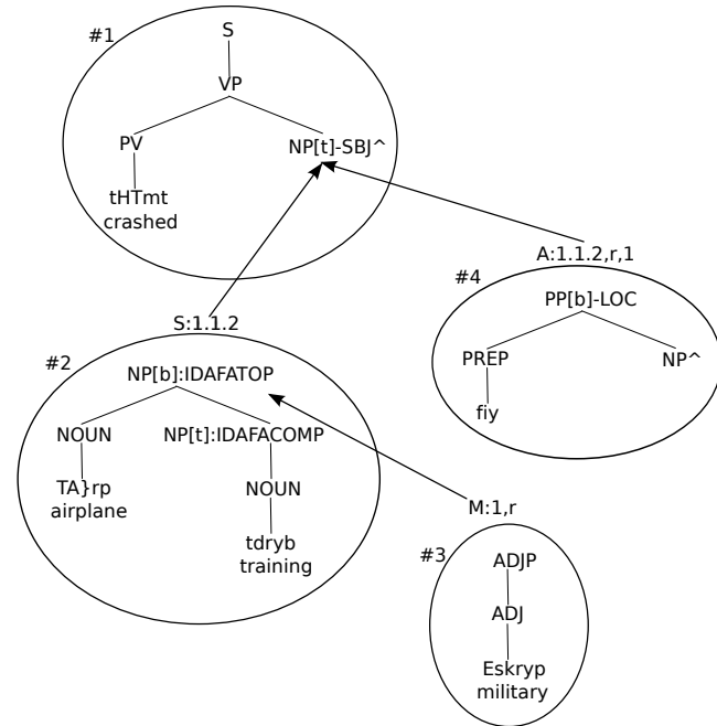
Figure 2: Elementary Trees and Derivation Tree for the Tree Decomposition in Figure 1
