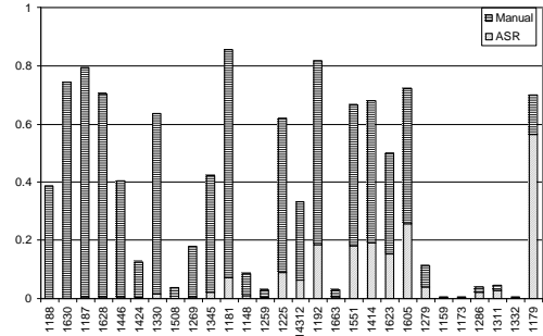
Figure 1: Average precision by topic, title queries. Full bar: Manual. Partial bar: ASR.
