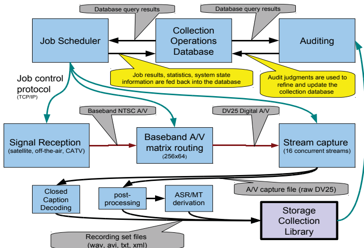
LDC Broadcast Collection Functional Block Diagram
